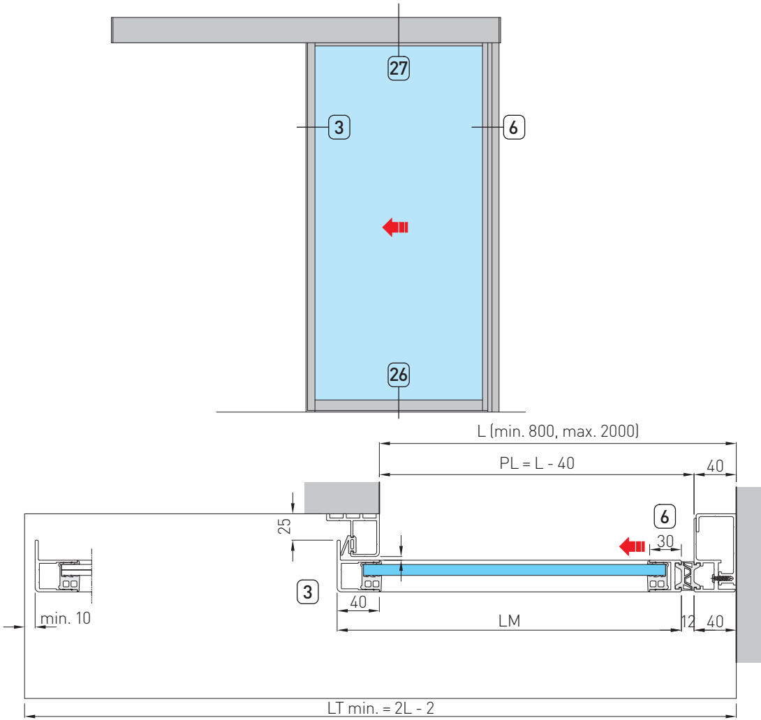
Horizontal section
