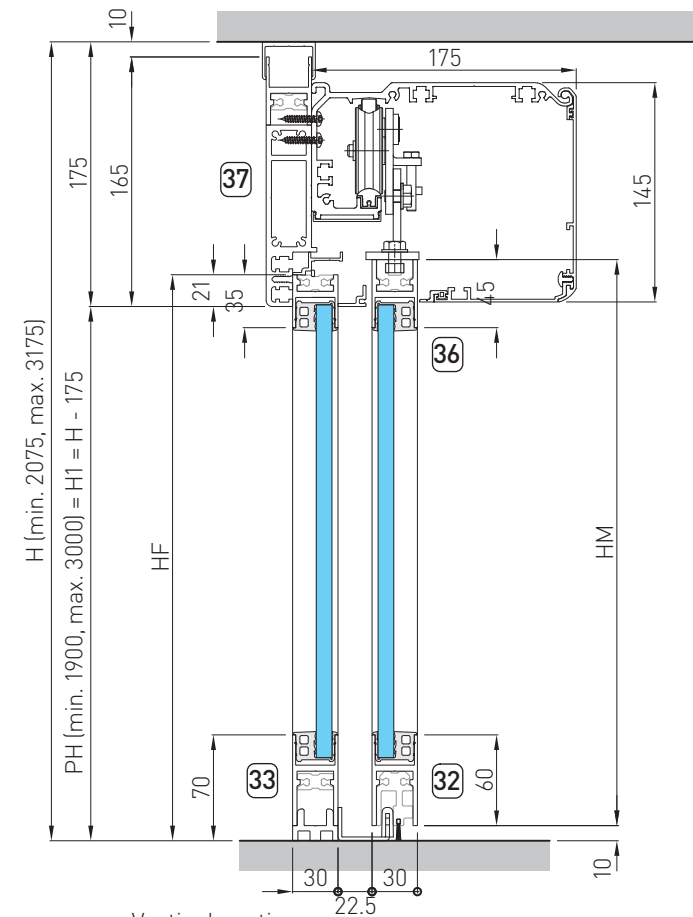
Vertical section
