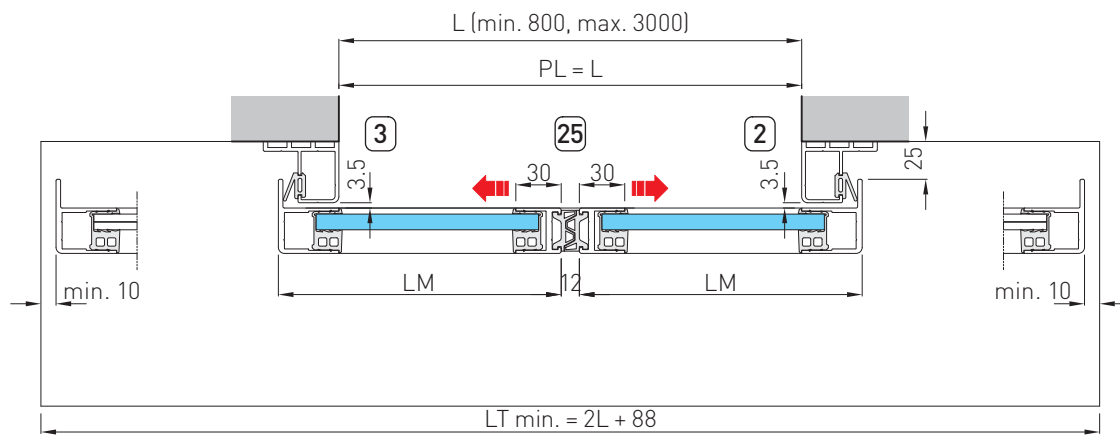
Horizontal section
