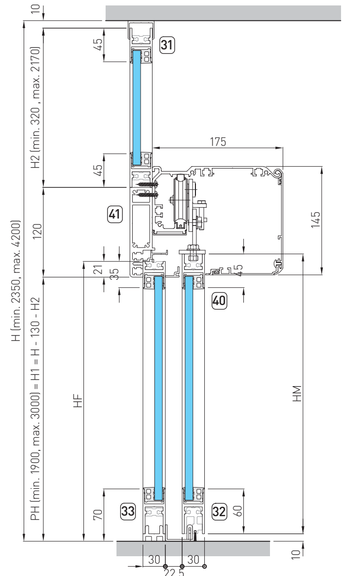
Vertical section
