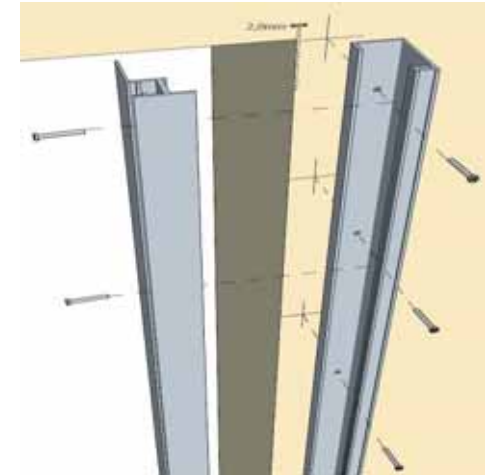
Post closing fixing
