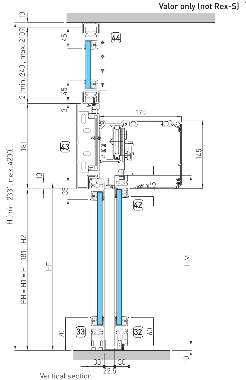
Vertical section
