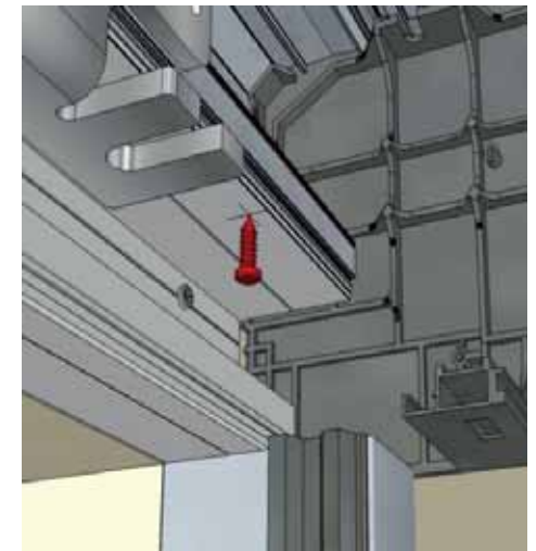
Operator fixing
