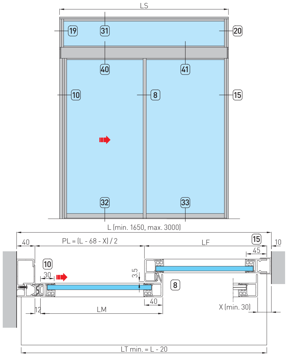
Horizontal section
