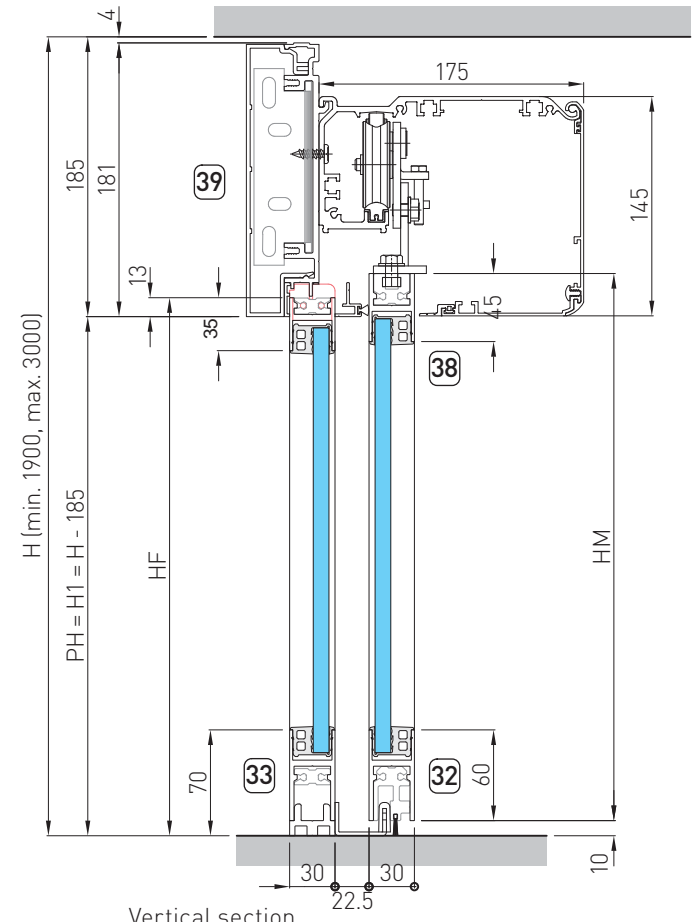
Vertical section
