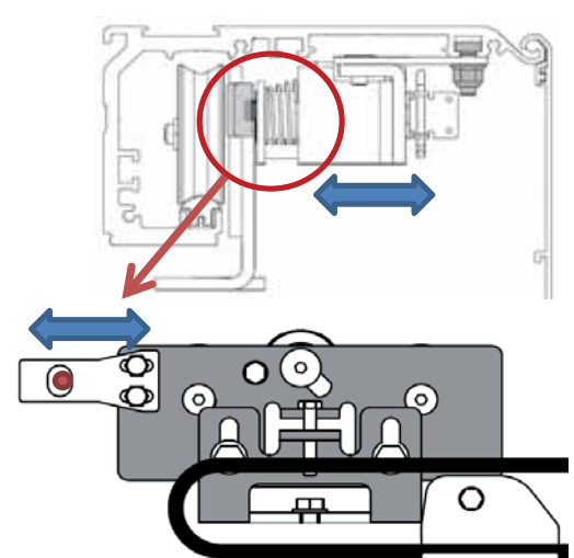
Electrolock adjustment
