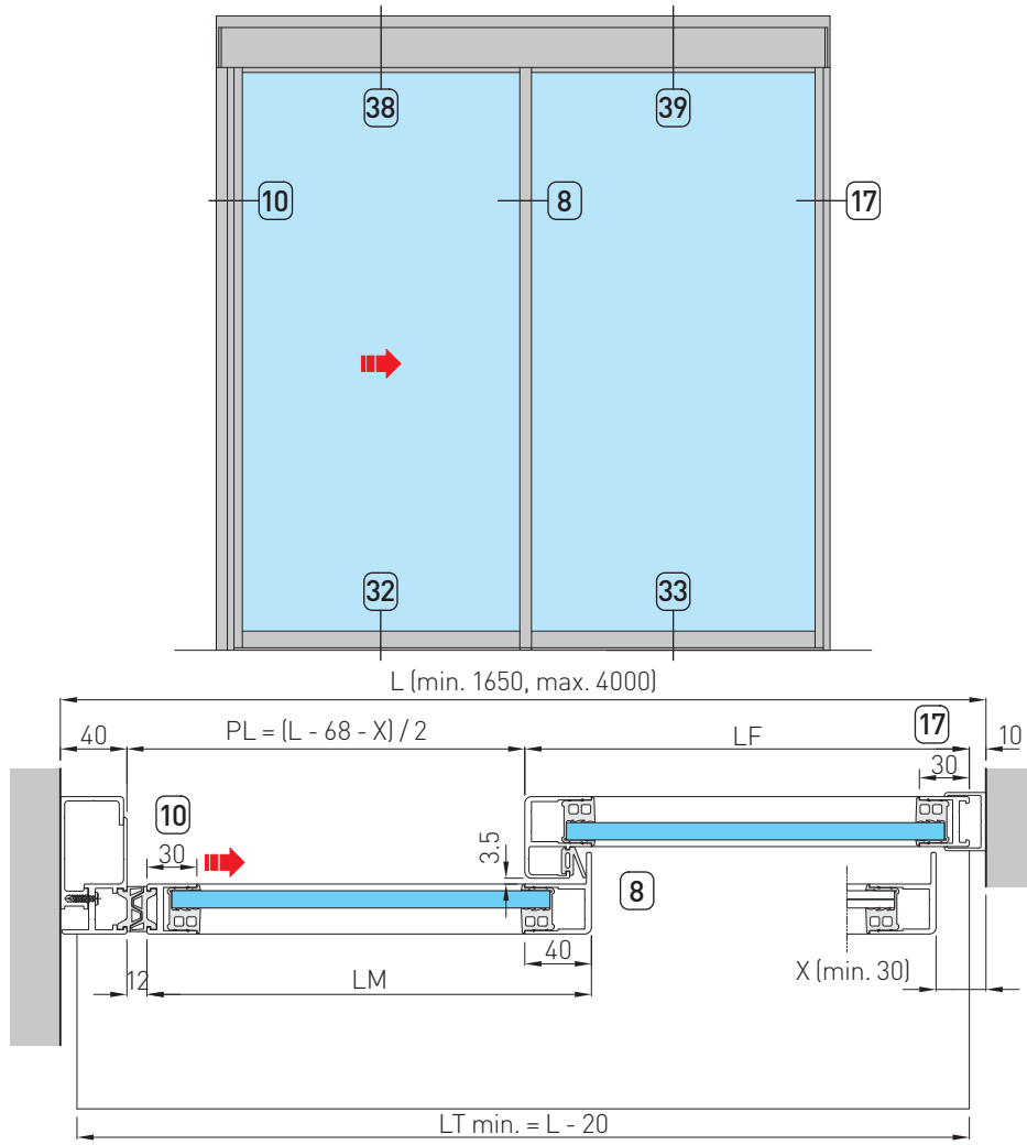
Horizontal section
