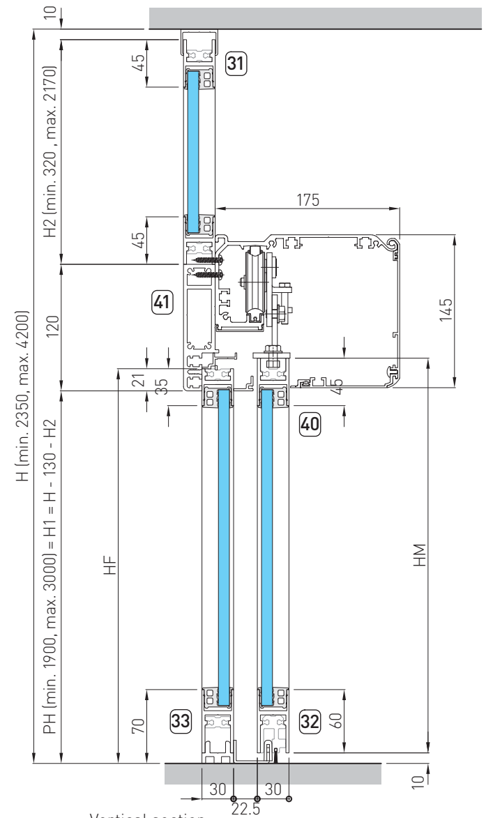
Vertical section
