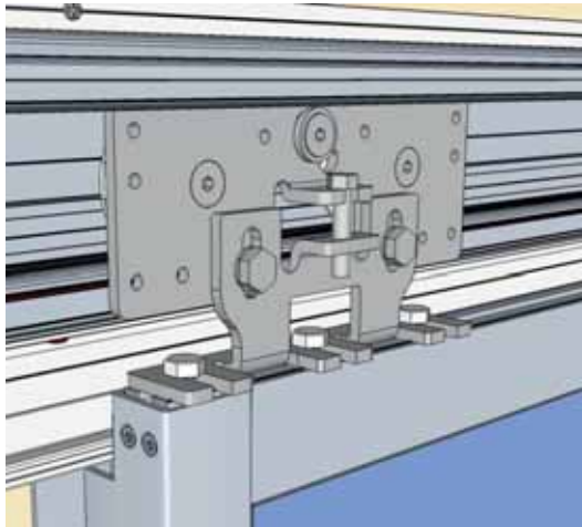
Mobile wing bracket fixing
