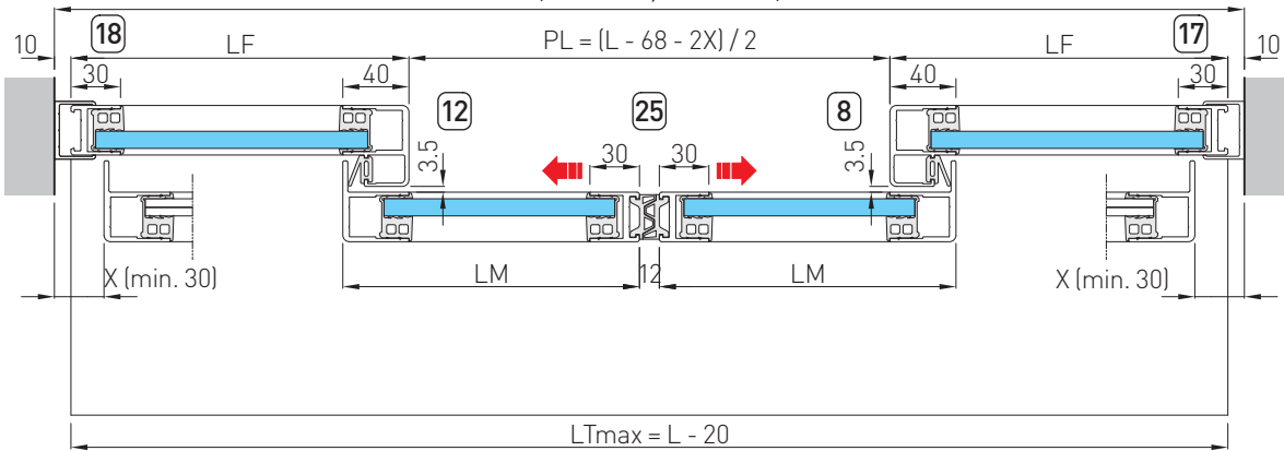
Horizontal section
