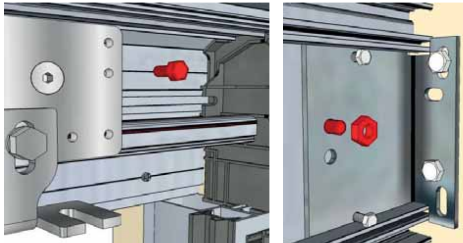
Operator fixing
