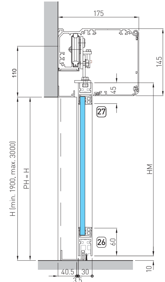
Vertical section
