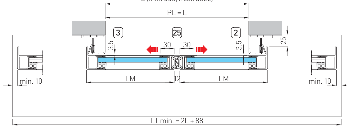
Horizontal section
