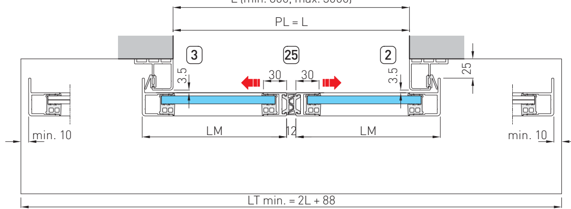
Horizontal section
