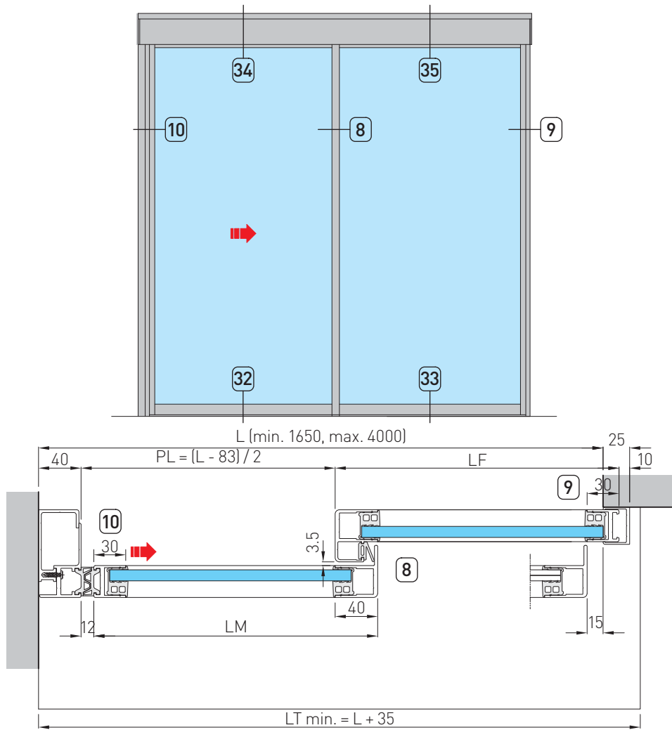
Horizontal section
