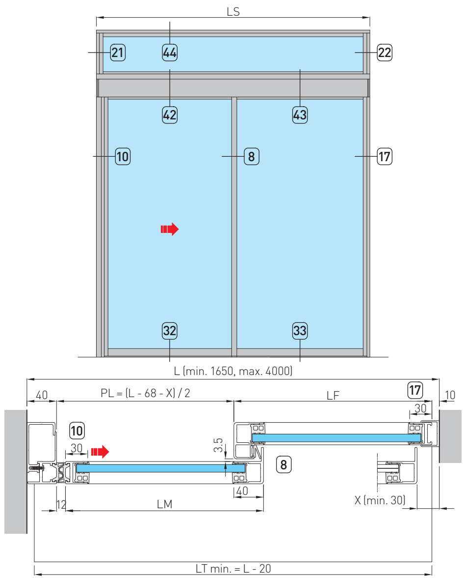
Horizontal section
