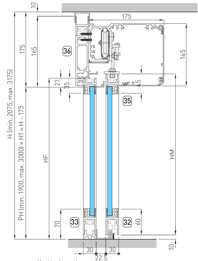
Vertical section
