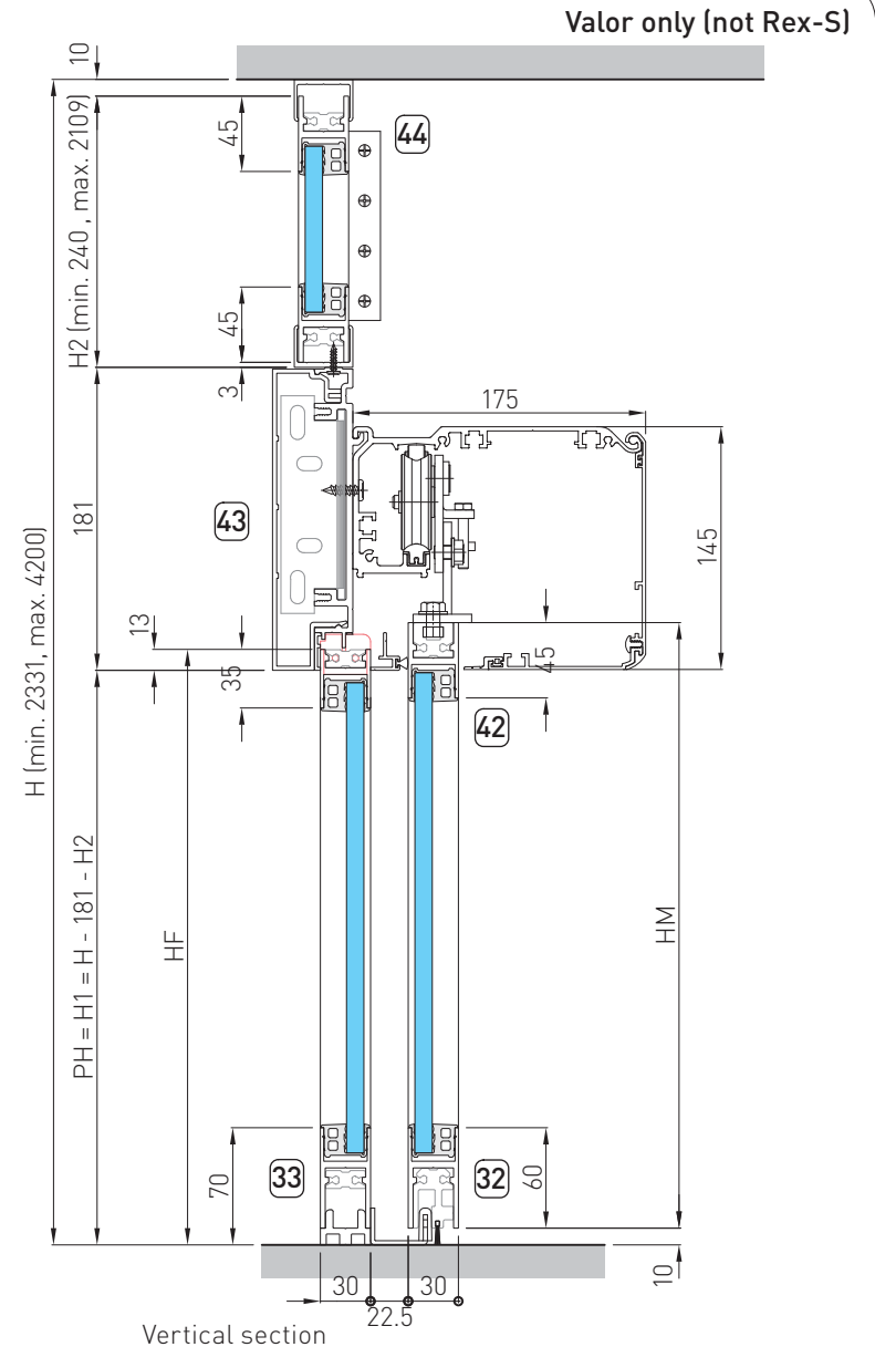
Vertical section
