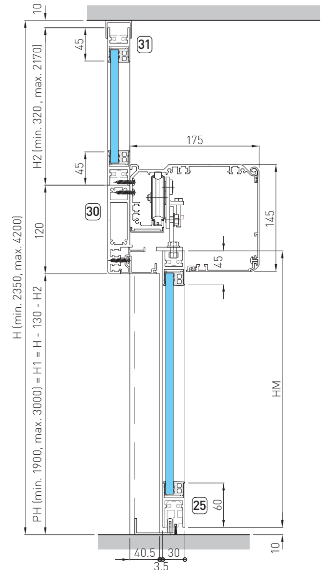
Vertical section
