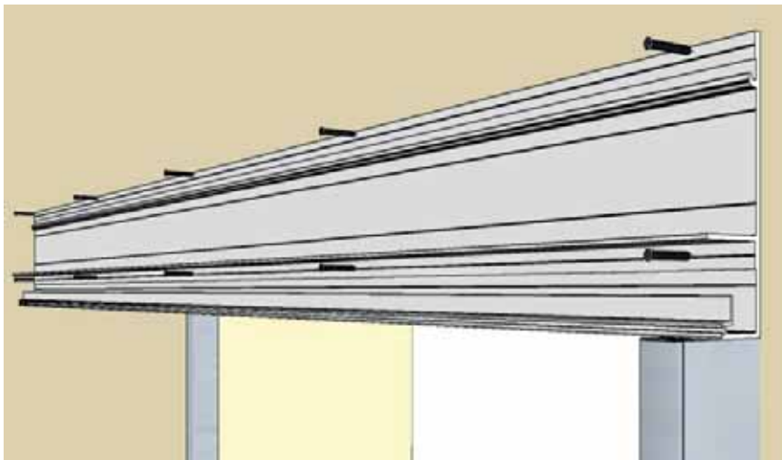
Simplified beam fixing
