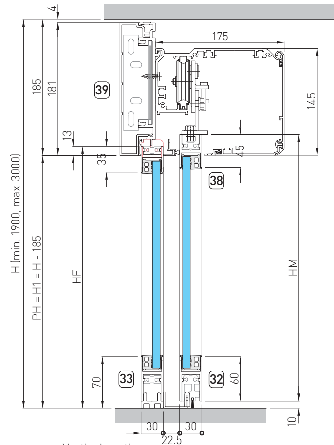
Vertical section
