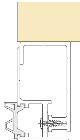
Section
