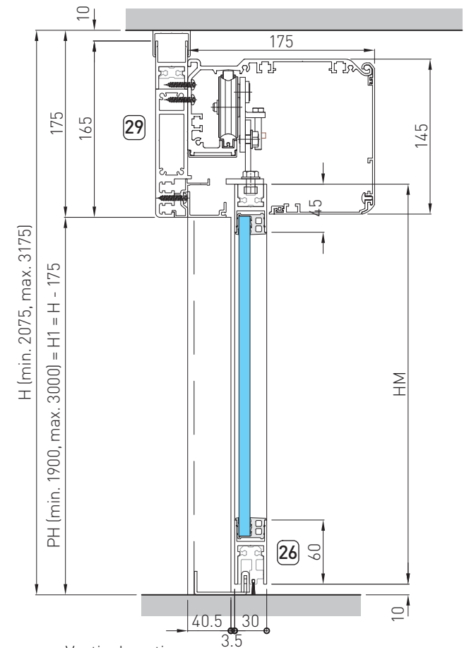
Vertical section
