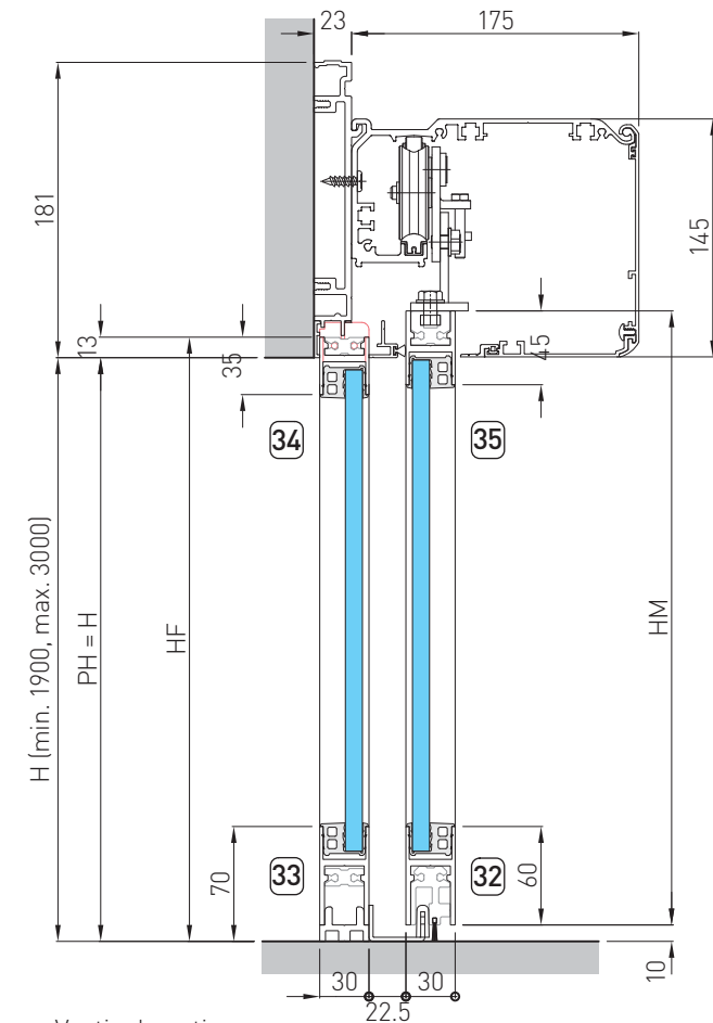
Vertical section
