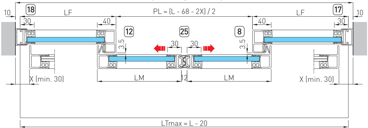
Horizontal section
