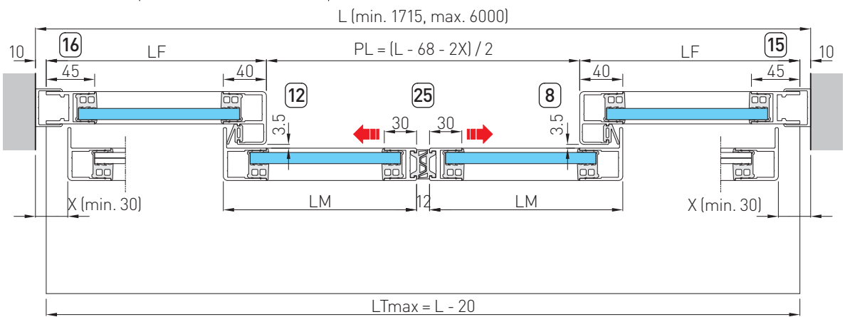
Horizontal section
