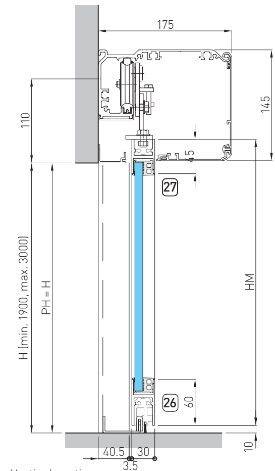
Vertical section
